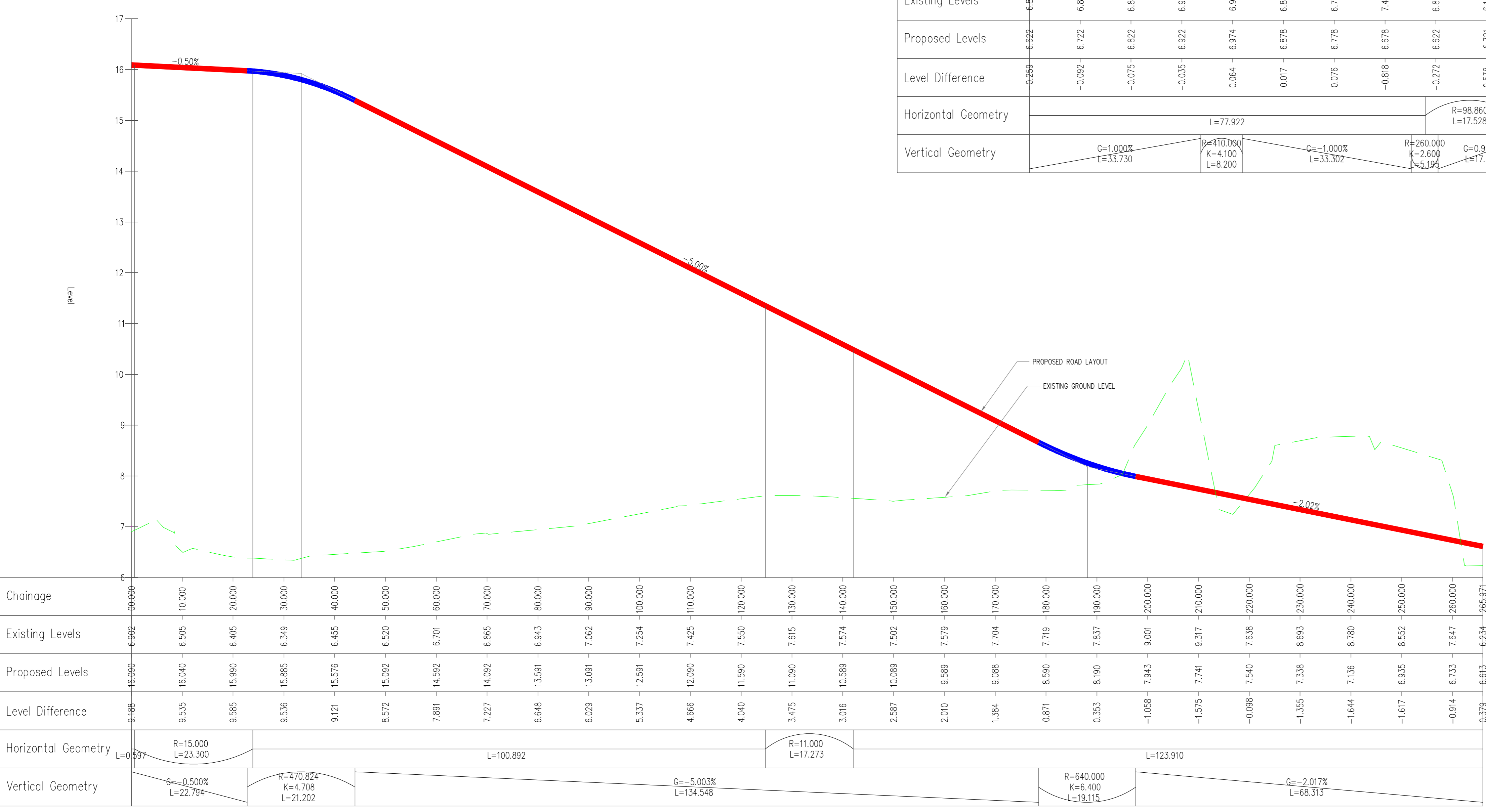
BUS ROUTE - LONGSECTION SCALE: H 1:500, V 1:50, DATUM: 6.000
